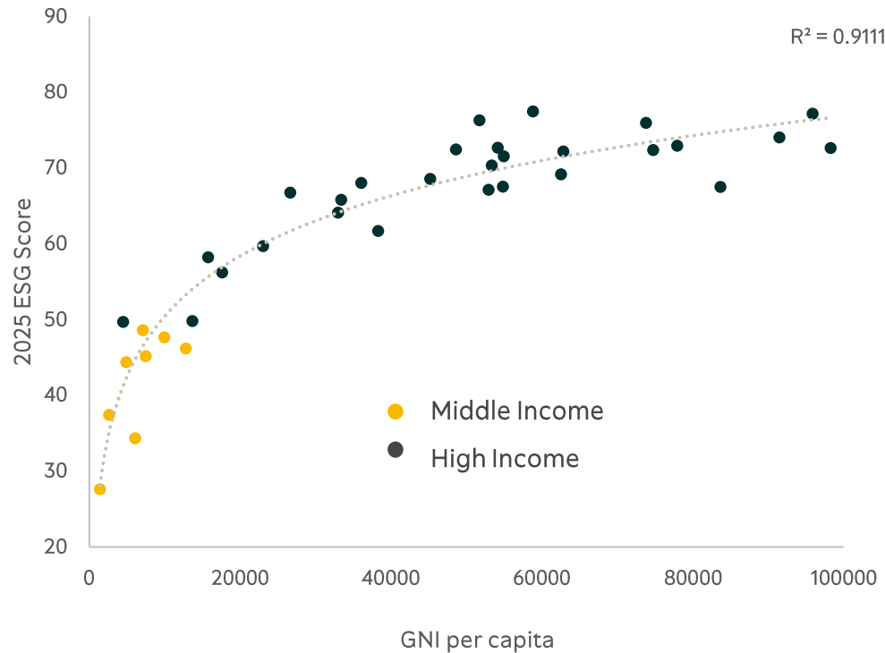
ESG Scores & Gross National Income
